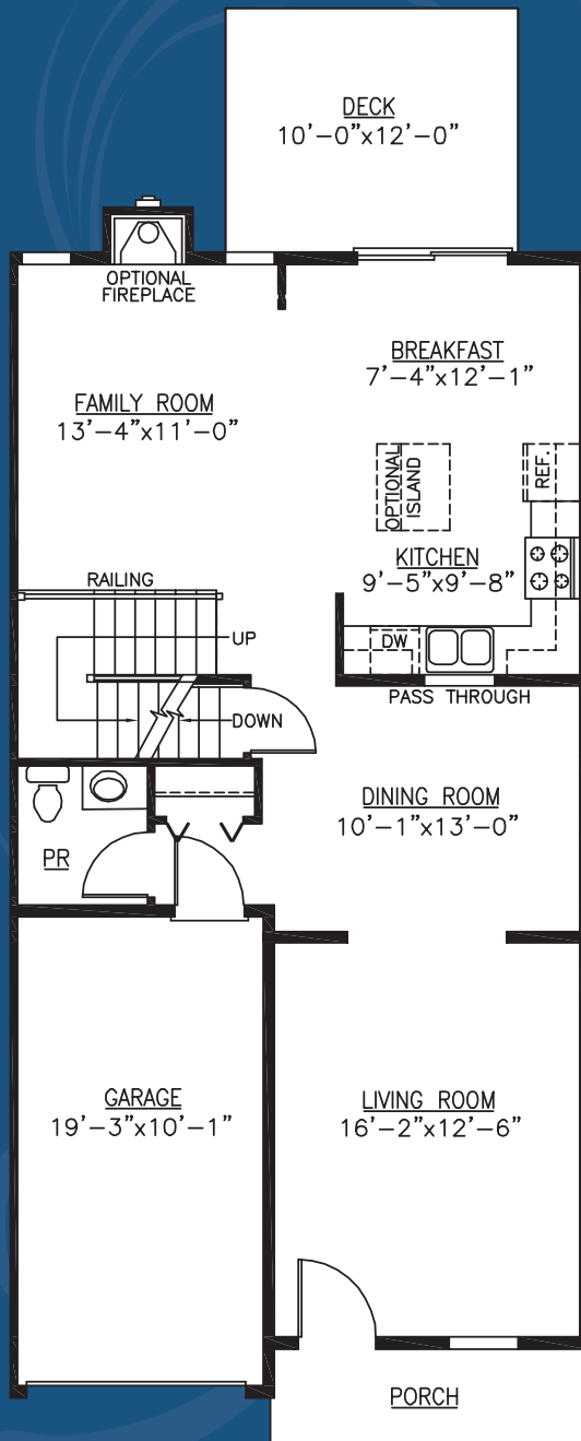
FIRST FLOOR
