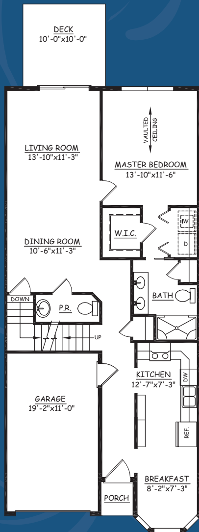
FIRST FLOOR
